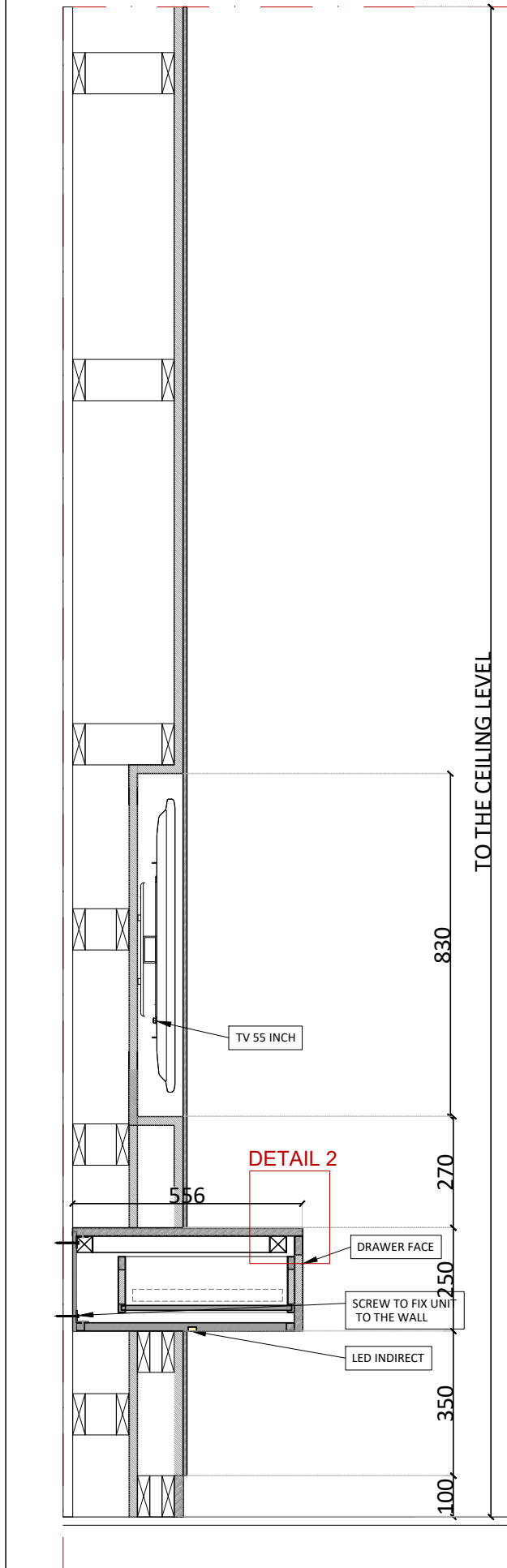
04 section aa
