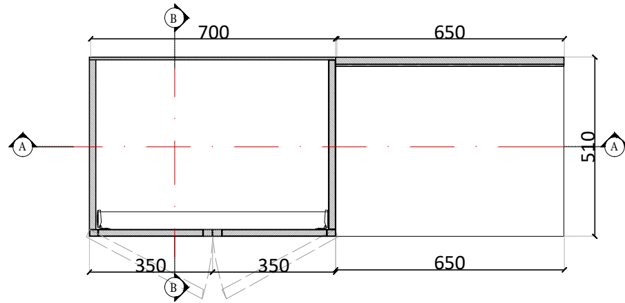
01 WARDROBE JW-MR-25 PLAN
