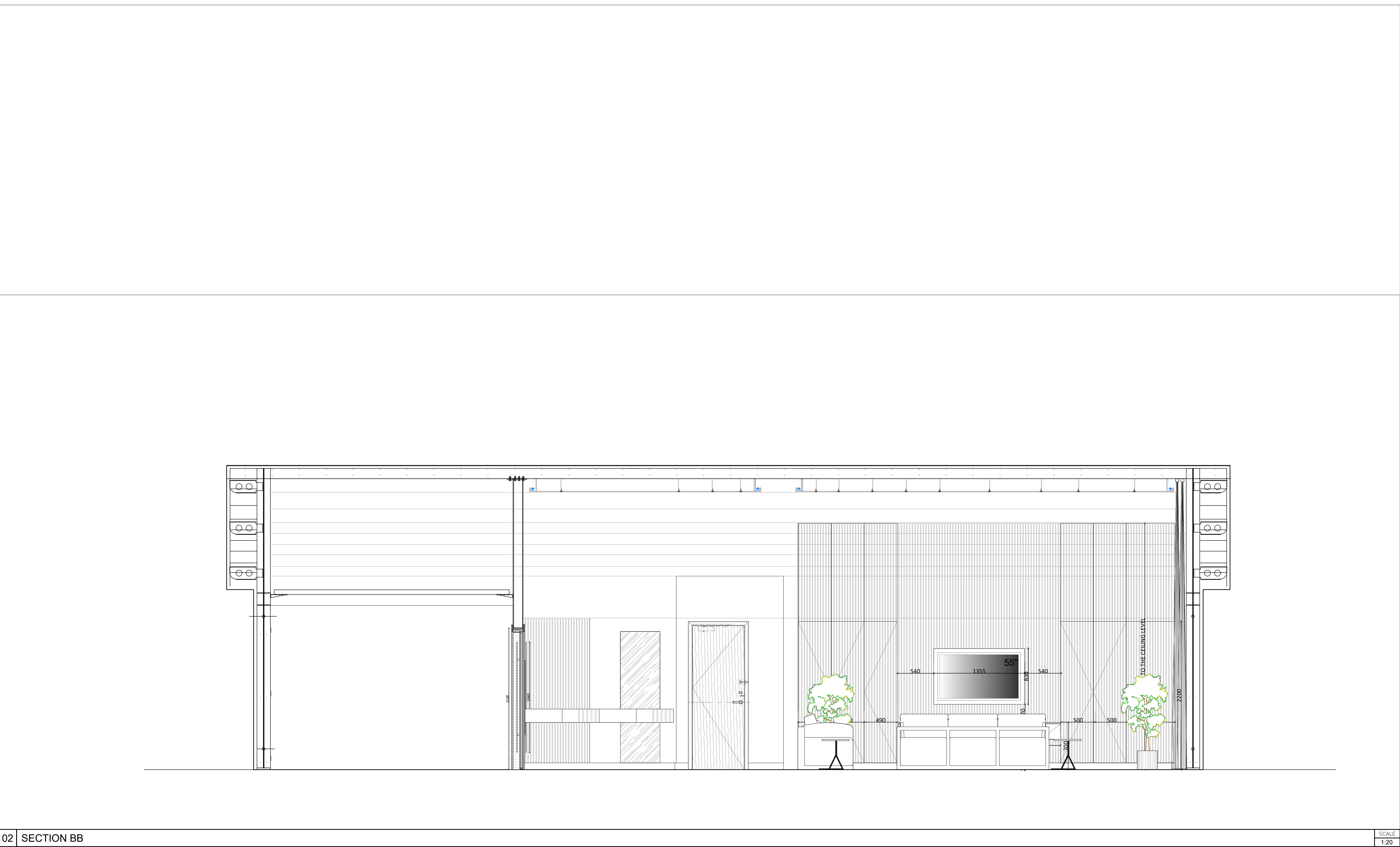
02 | SECTION BB
