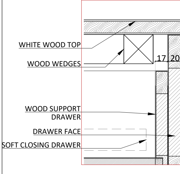
06 Detail 02
