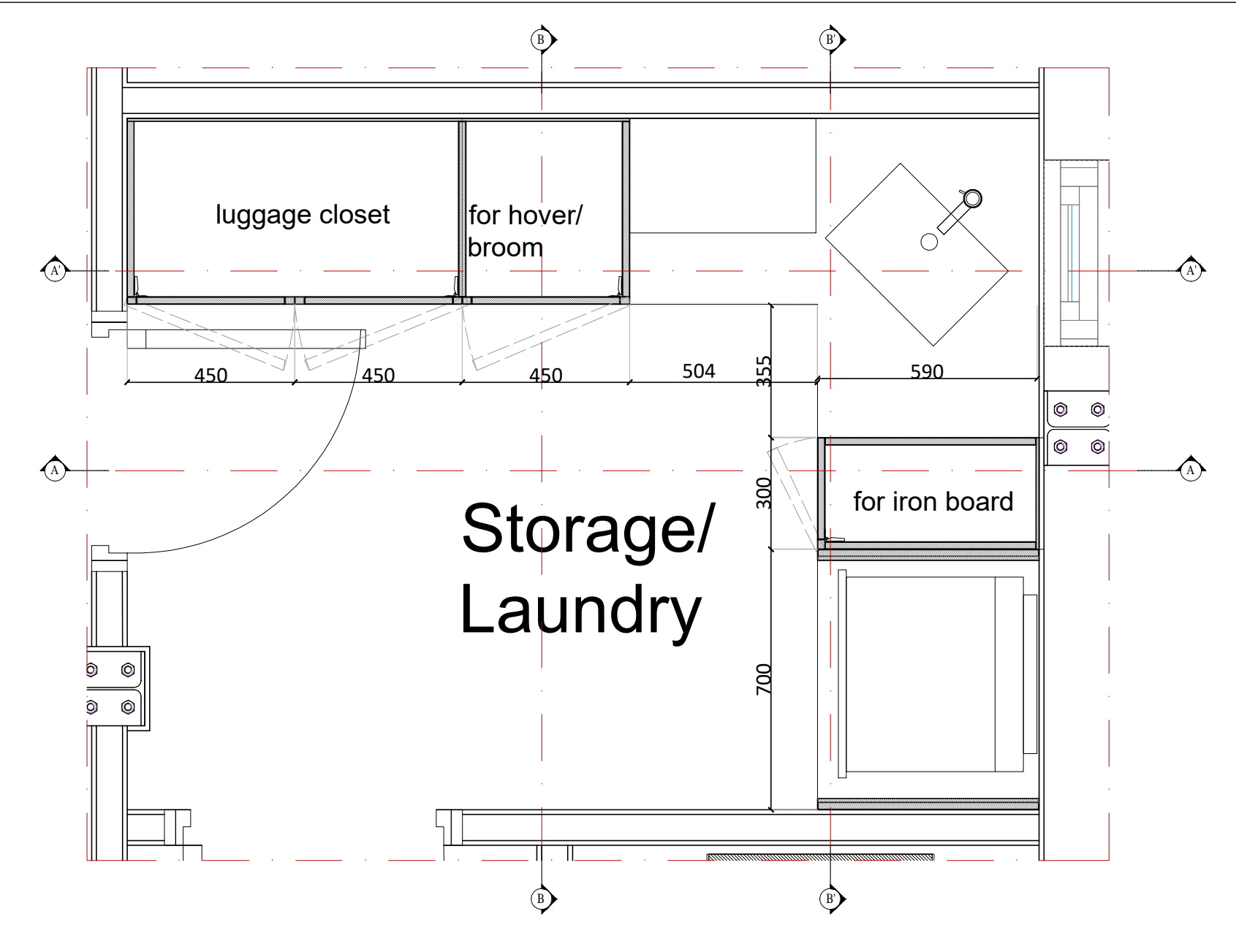
01 LAUNDRY AND STORAGE JW-S-19 PLAN
