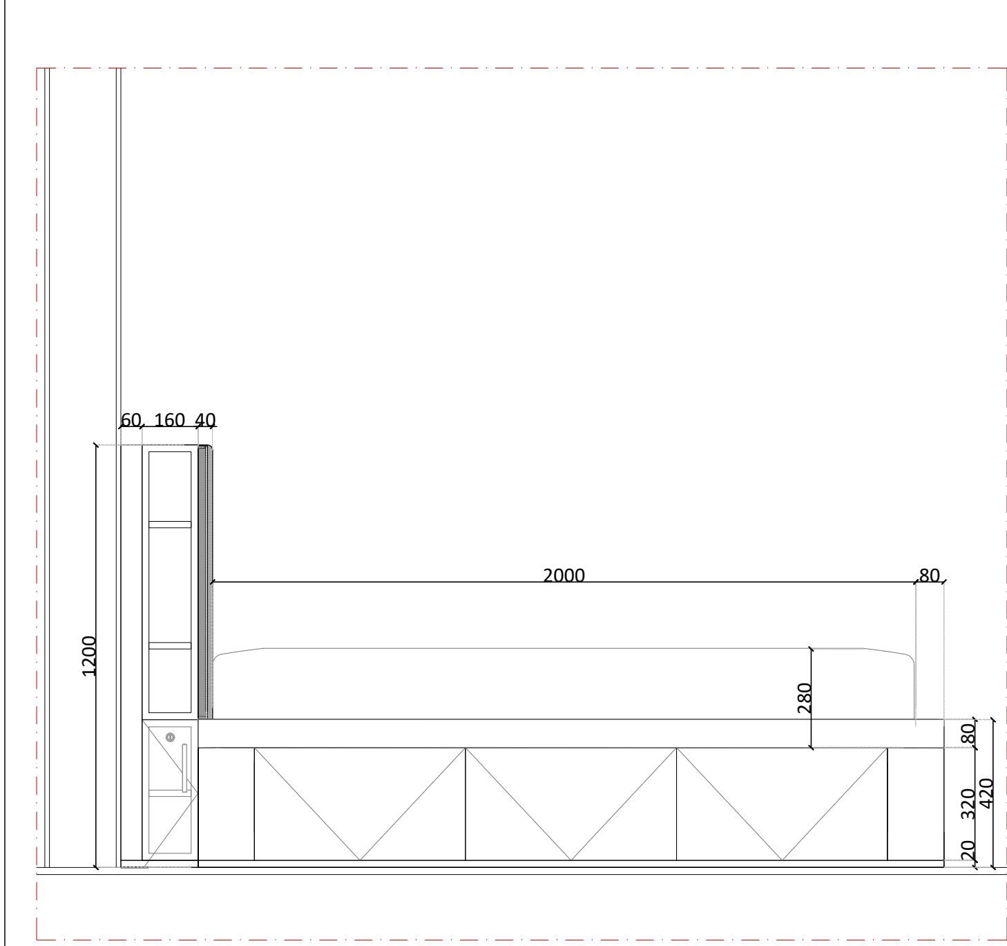
04 HEADBOARD SIDE VIEW
