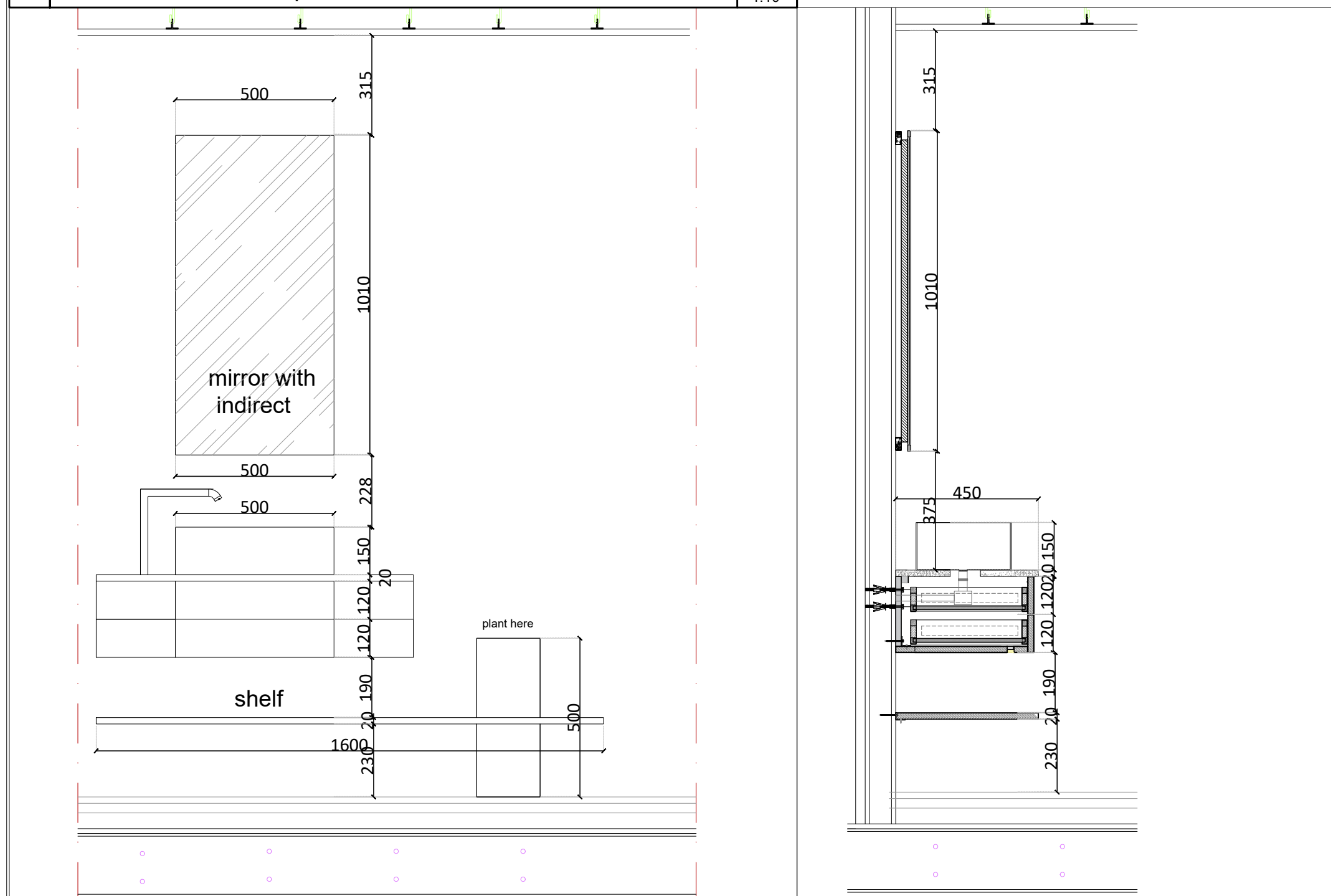
10 | VANITY JW-GB-09 FRONT VIEW 11 | VANITY JW-GB-09 SECTION AA
