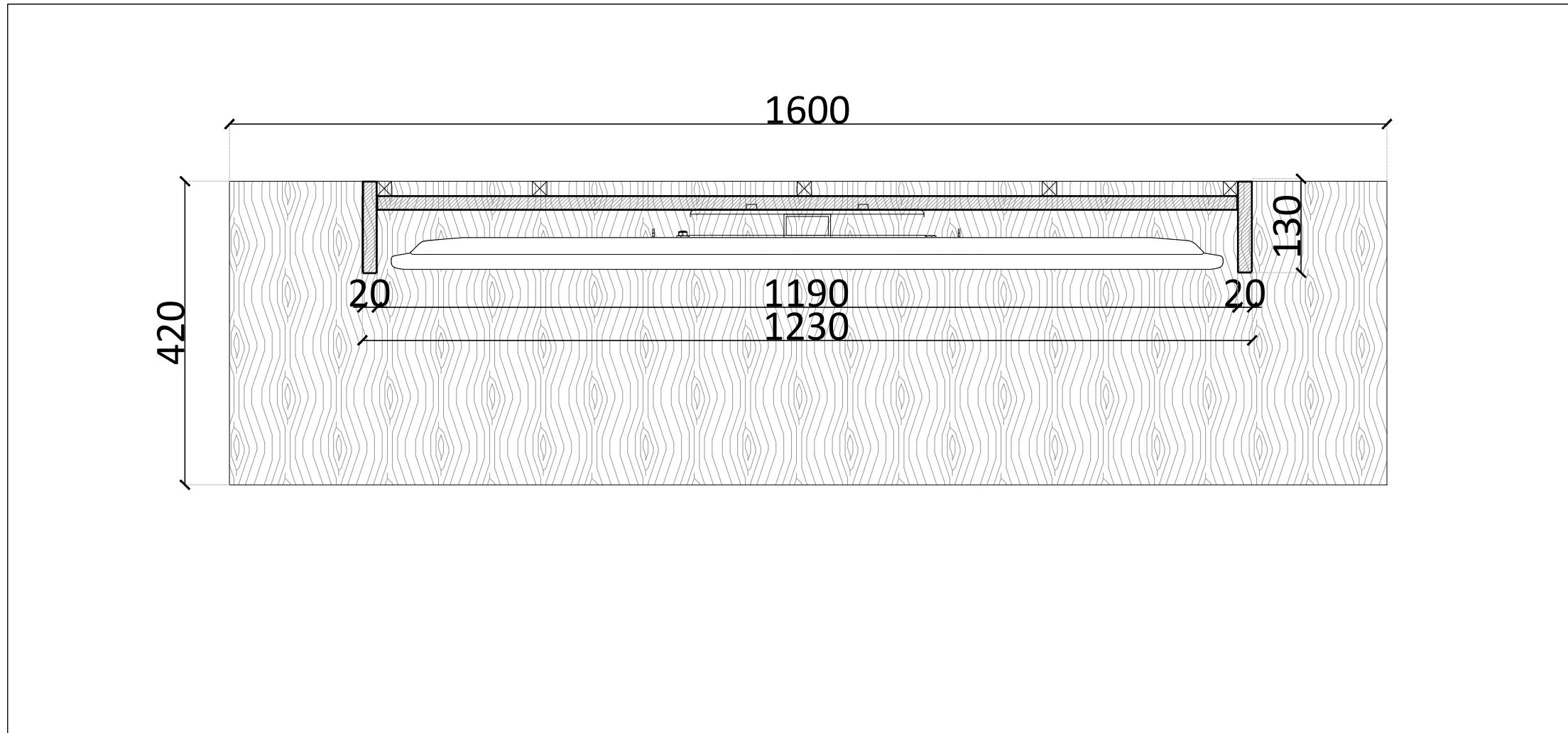
01 tv unit top view
