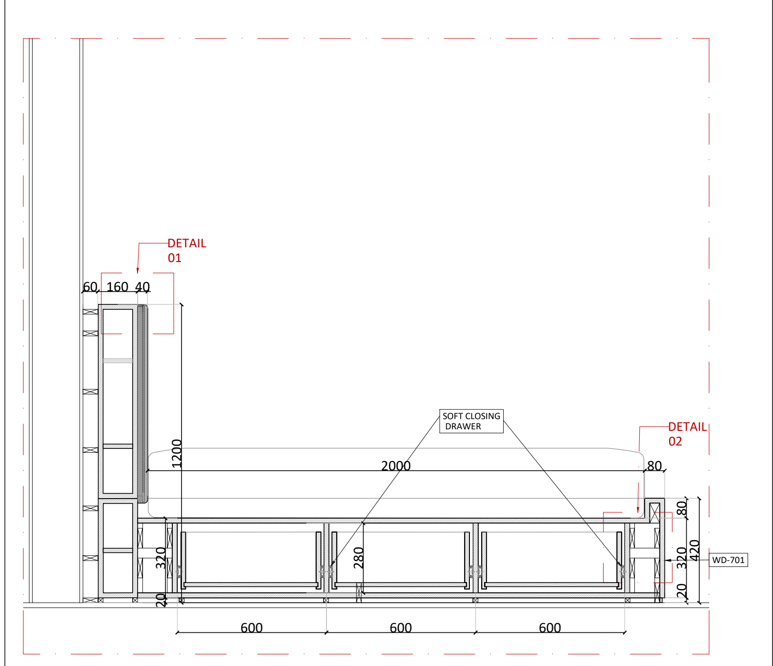
03 HEADBOARD SECTION A
