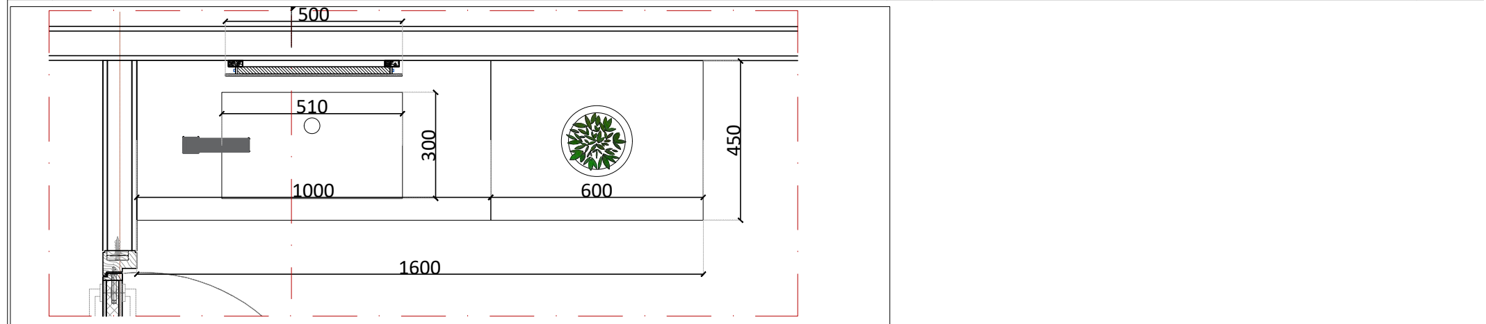
09 | VANITY JW-GB-09 top view
