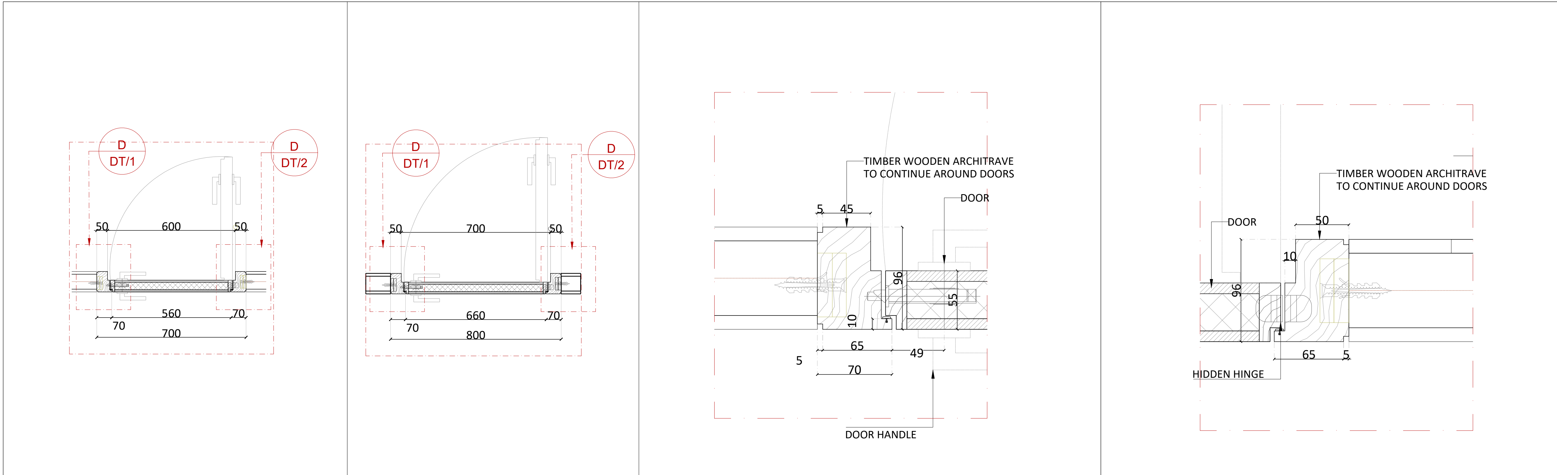
01PLAN JW-MB-21SCALE1:10 01'PLAN JW-MB-20SCALE1:10 04DETAIL 01SCALE1:2 05DETAIL 02SCALE1:2
