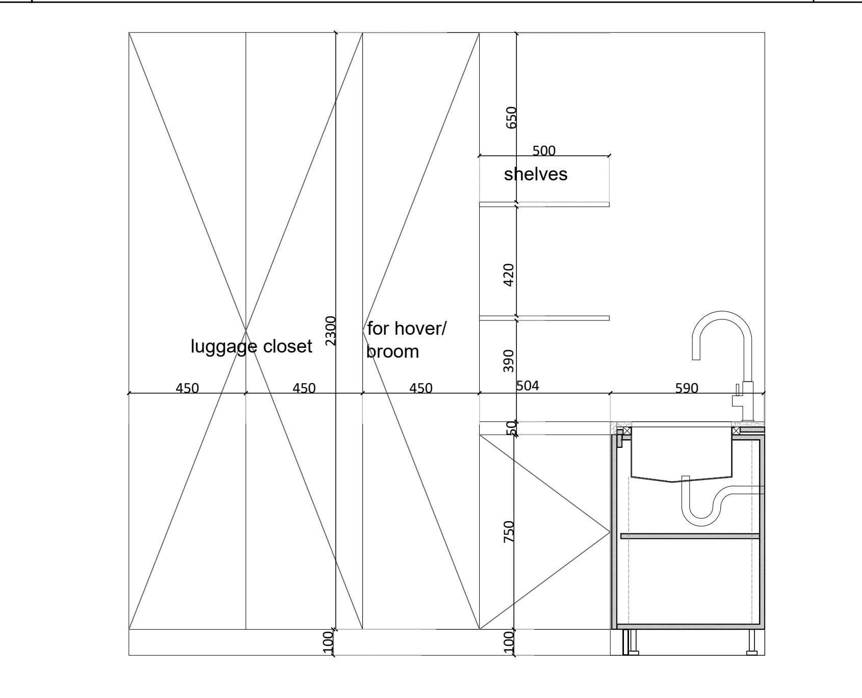
02 SECTION A LAUNDRY AND STORAGE JW-S-19
