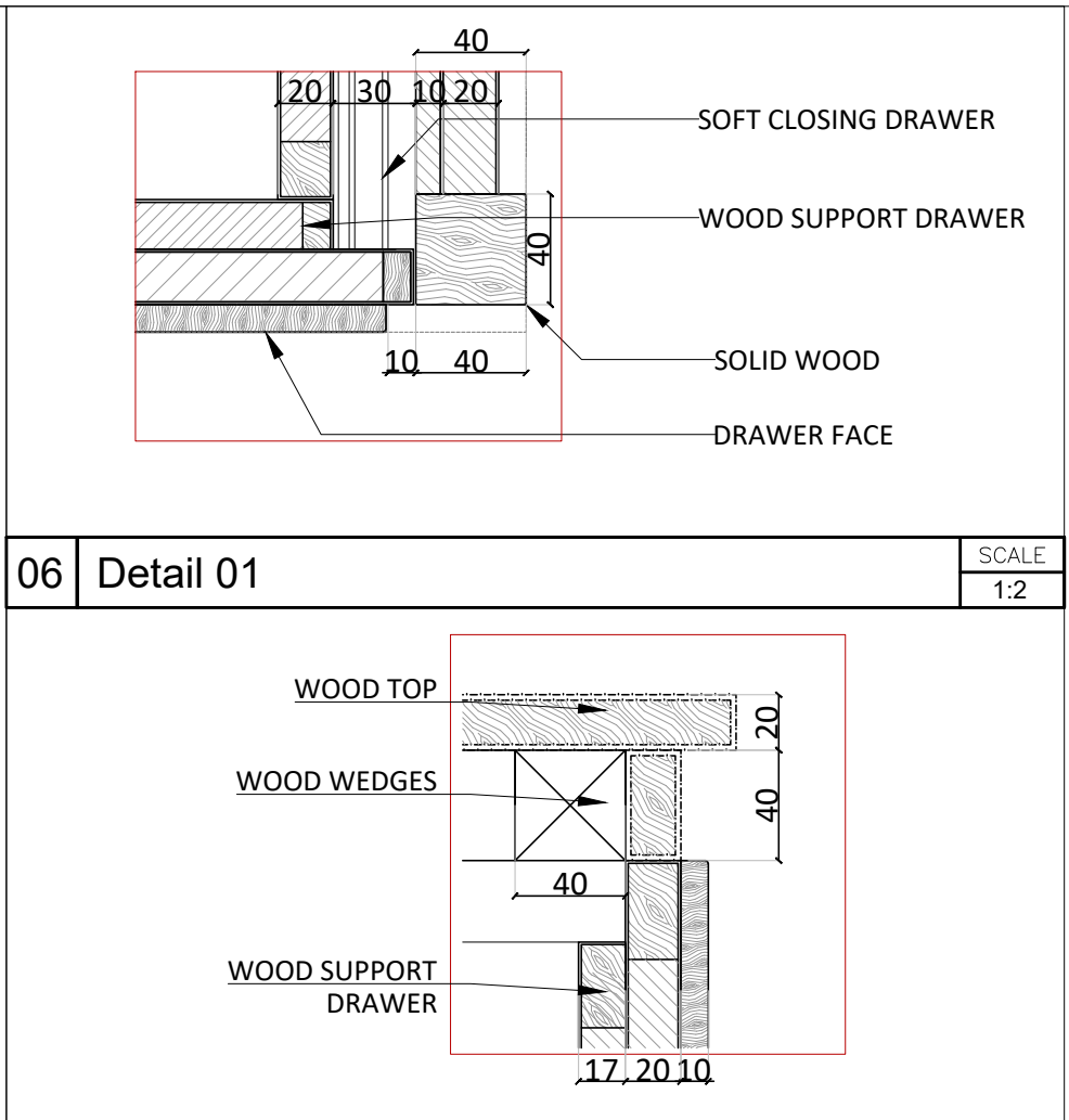
06 Detail 01
