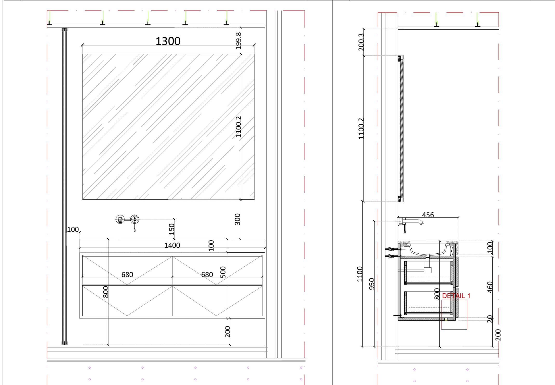
02 | FRONT VIEW VANITY JW-MB-10 03 | SECTION AA JW-MB-10
