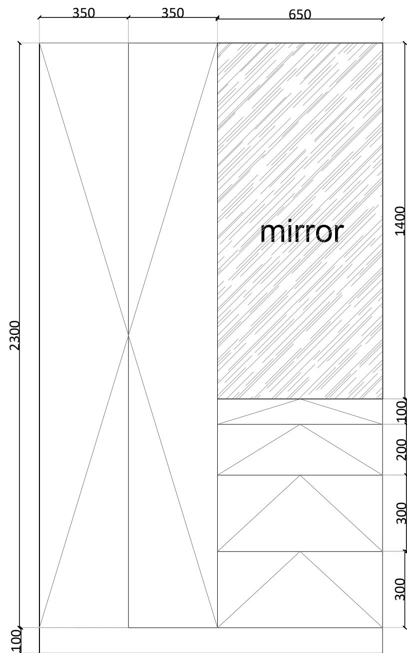
02 FRONT VIEW JW-MR-25
