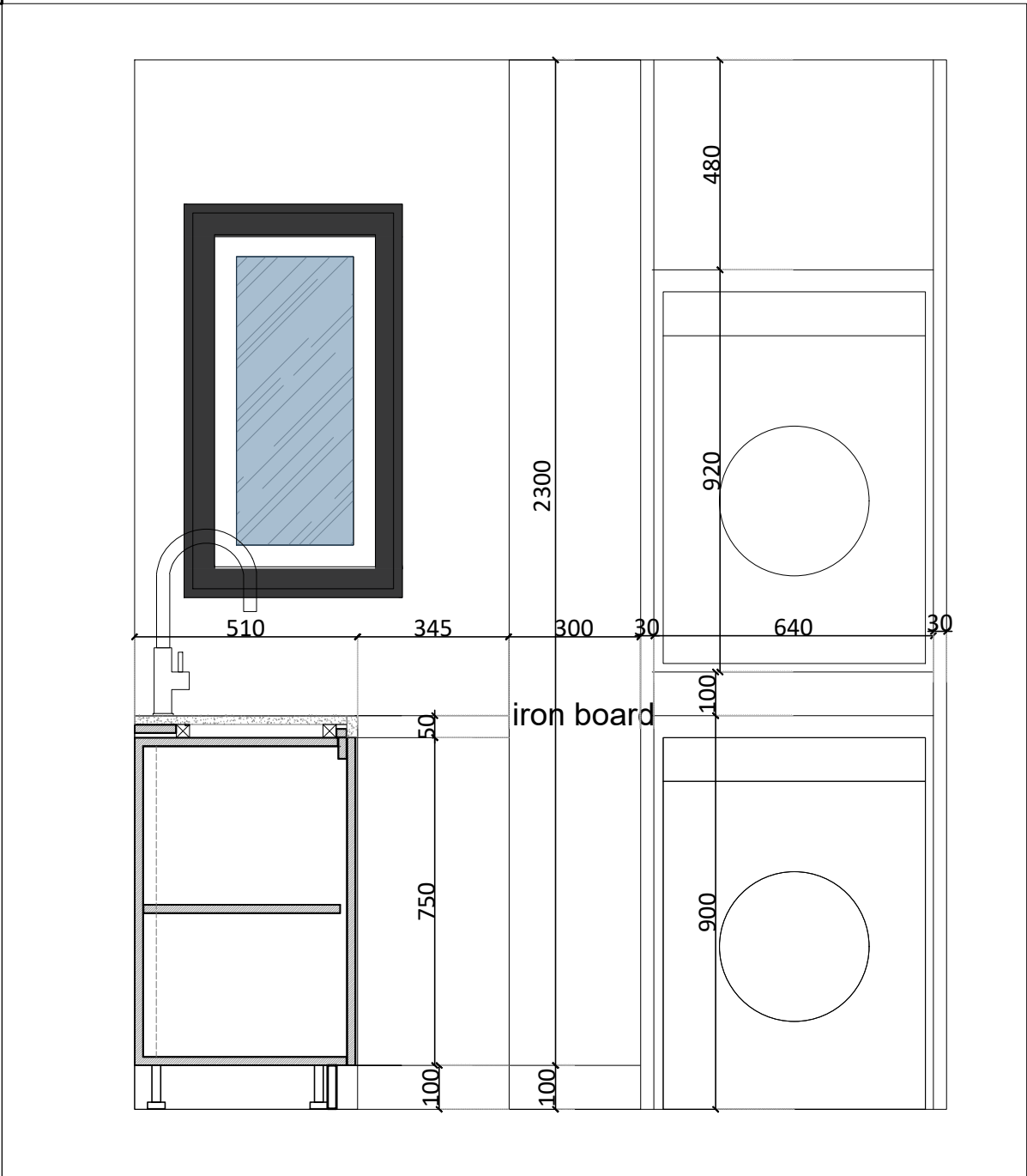
05 SECTION BB' LAUNDRY AND STORAGE JW-S-19
