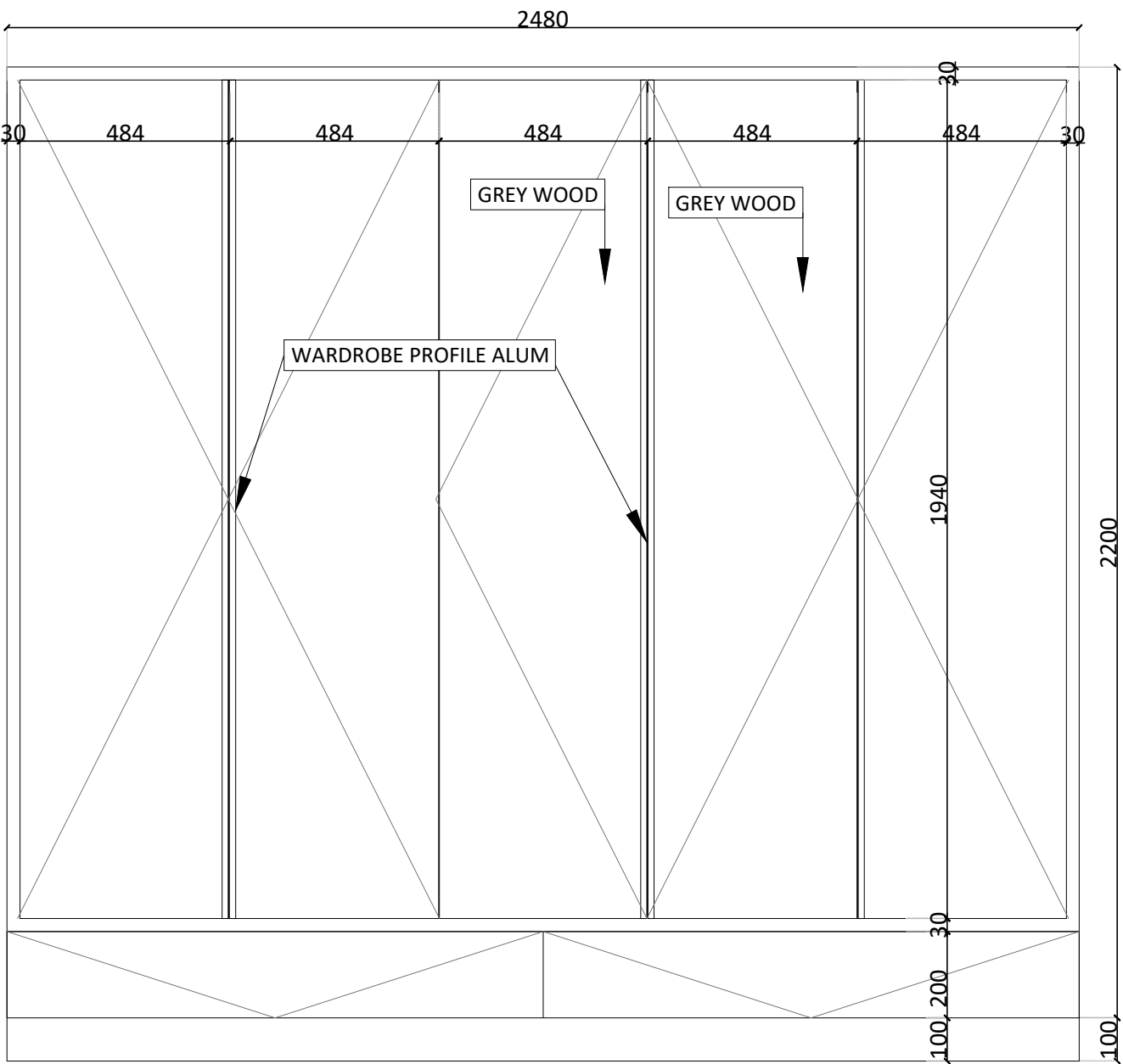
02 FRONT VIEW JW-MB-13
