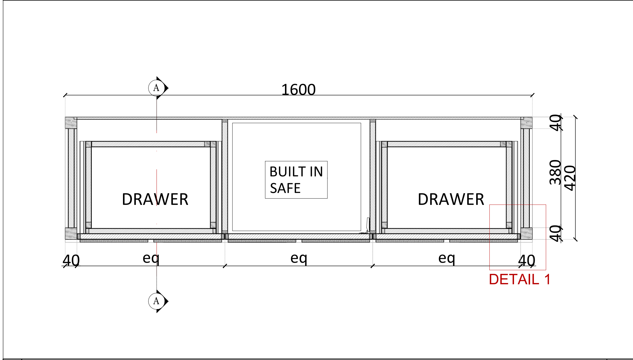
02 tv unit plan
