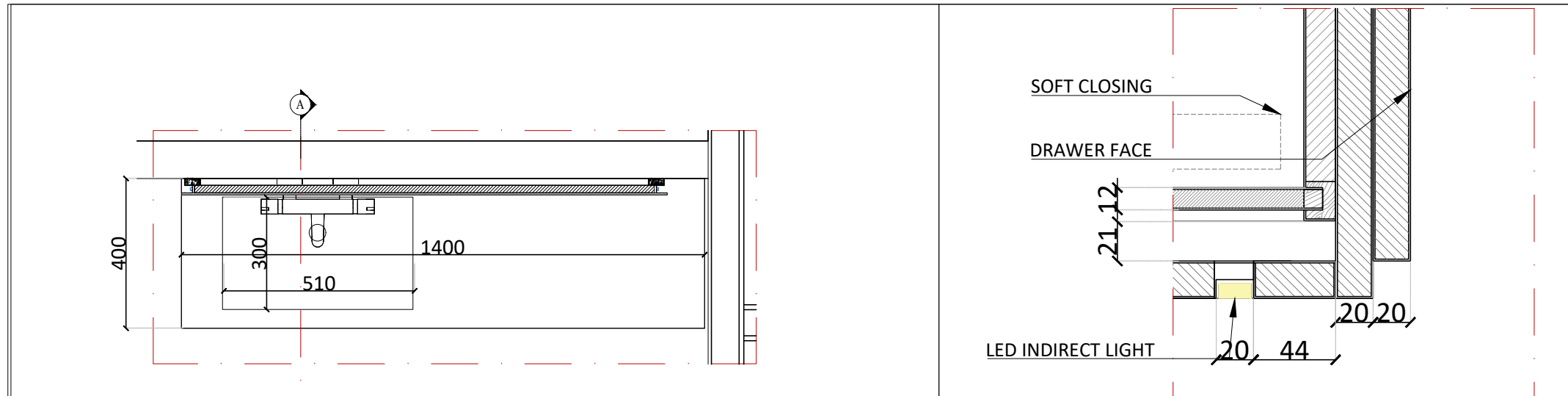
01 | VANITY JW-MB-10 top view 04 | DETAIL 01 JW-MB-10
