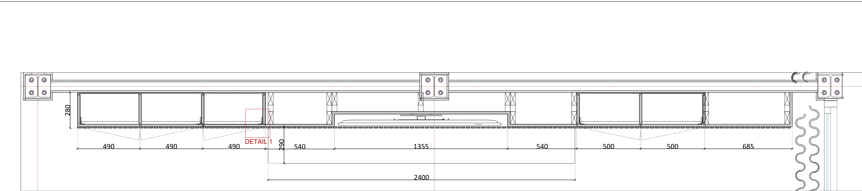
01 tv unit top view
