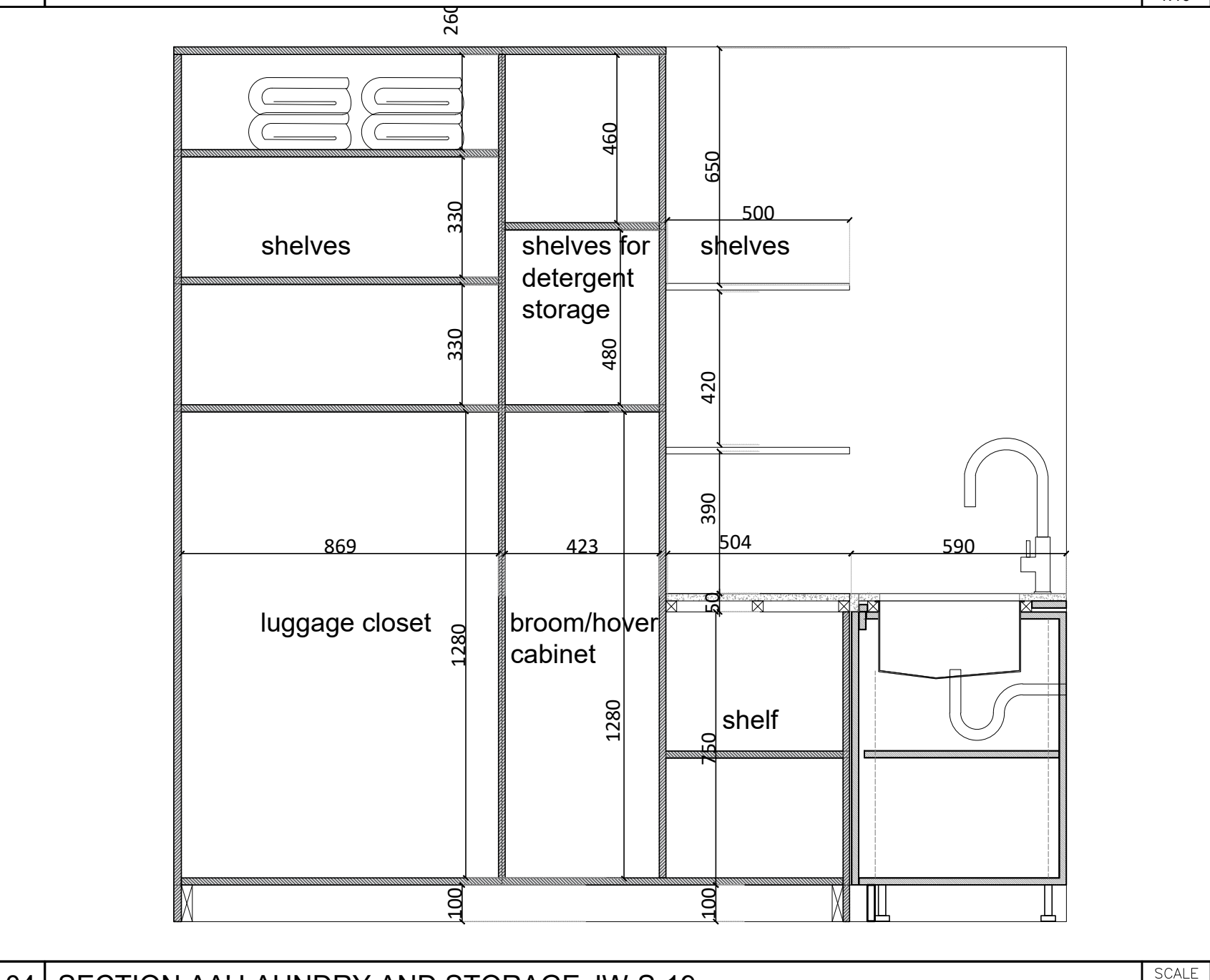
04 SECTION AA' LAUNDRY AND STORAGE JW-S-19
