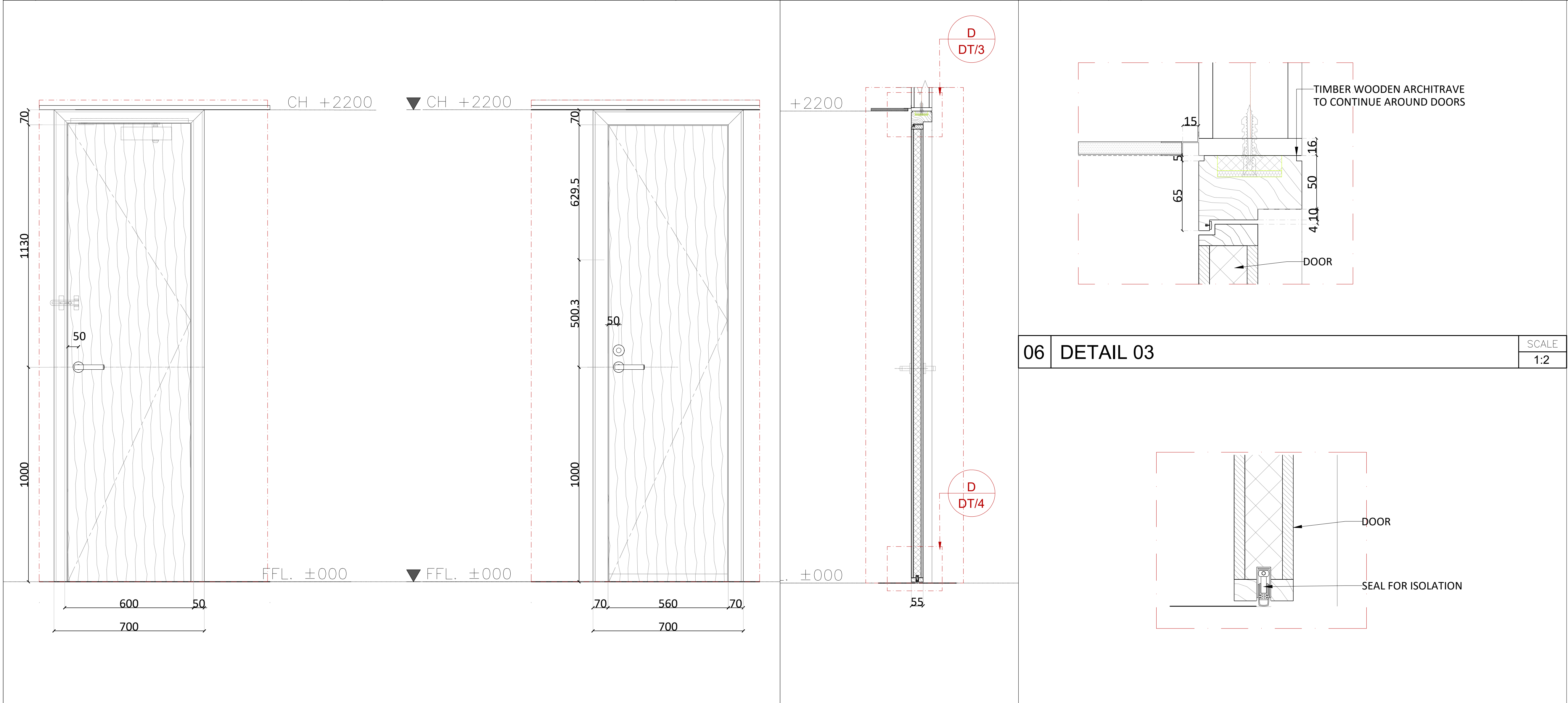
02ELEVATIONSCALE1:10 03SECTION AASCALE1:10 07DETAIL 04SCALE1:2
