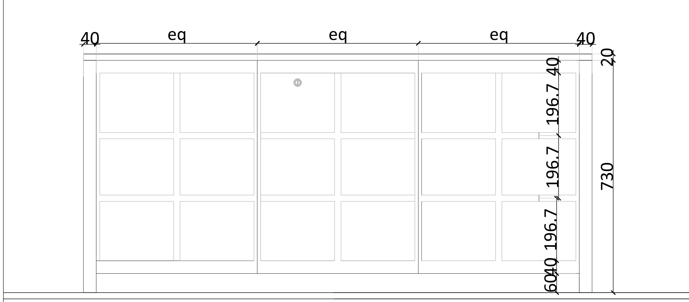
03 tv unit FRONT VIEW
