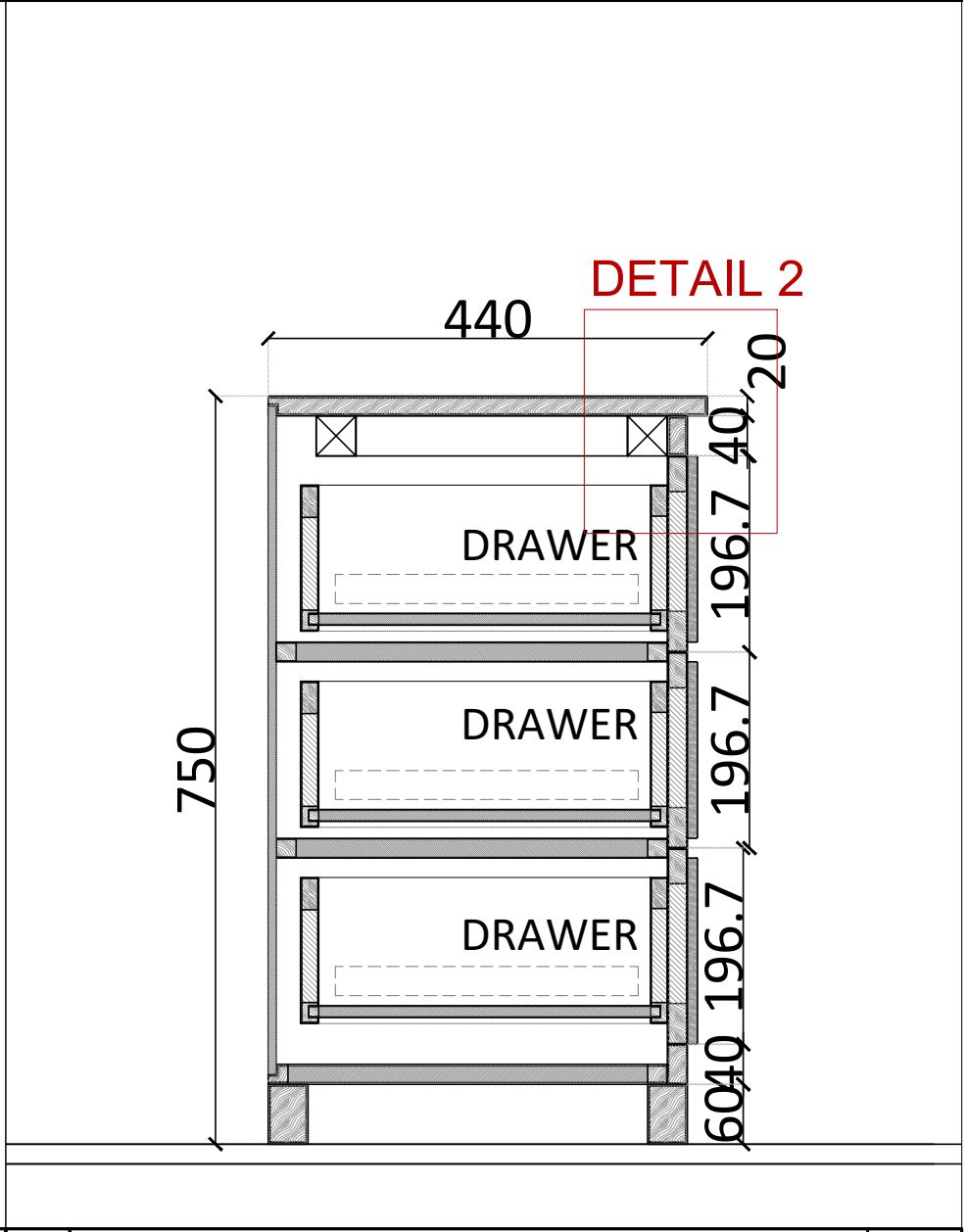
04 tv unit section A
