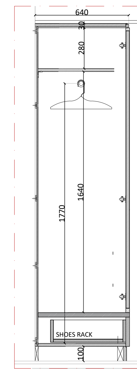
04 SECTION B
