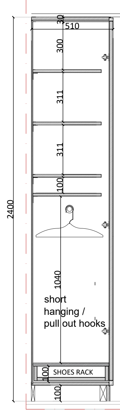
04 SECTION BB
