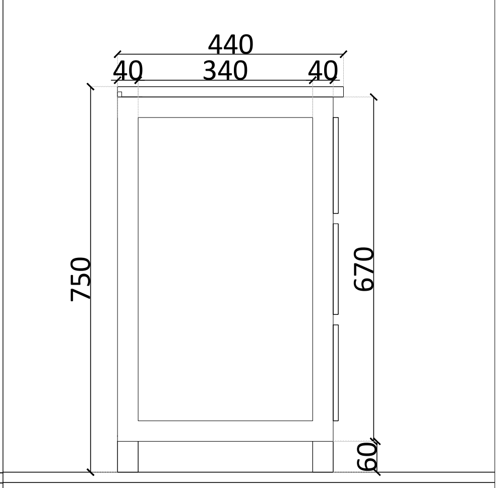
05 SIDE VIEW
