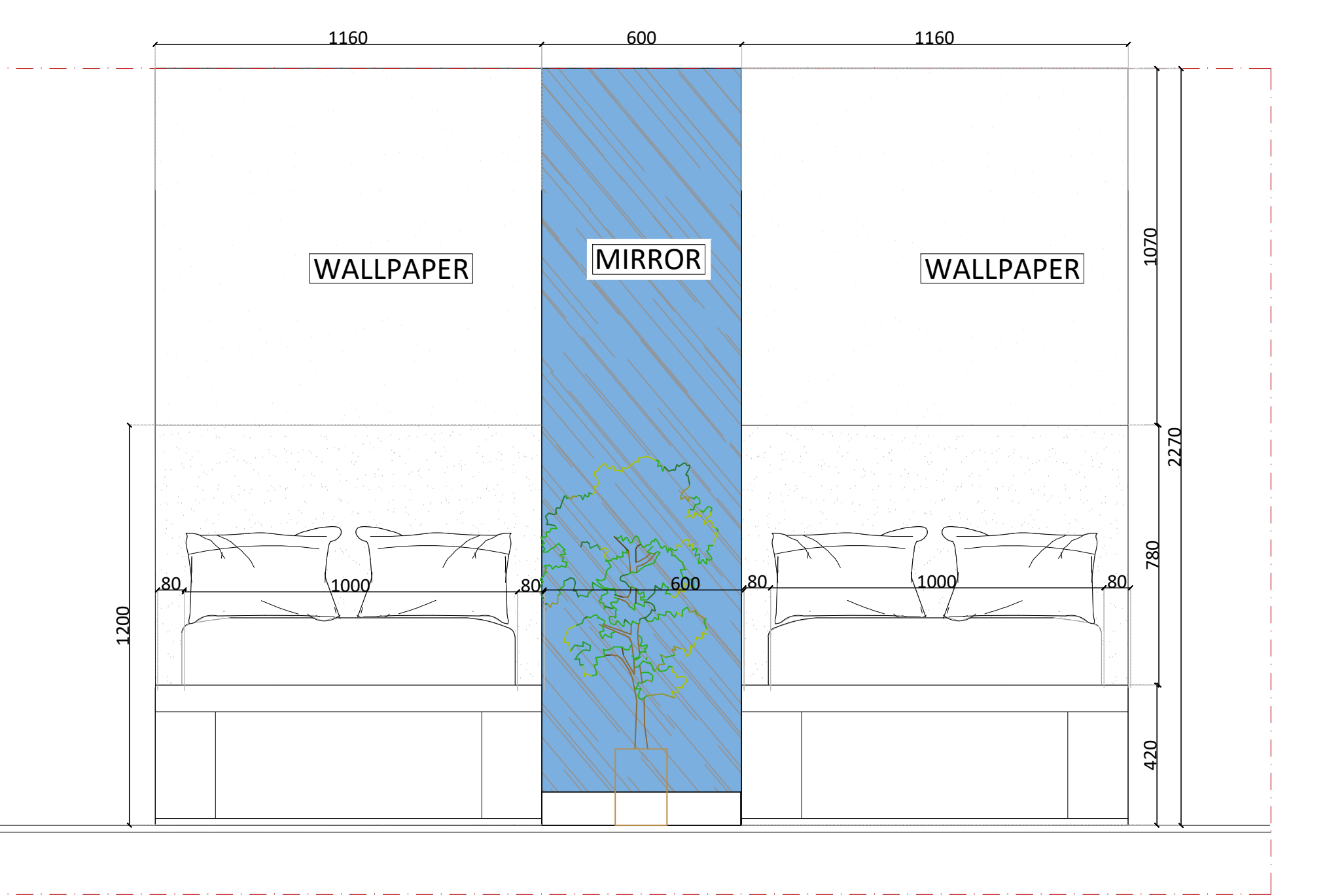
01 HEADBOARD JW-MB-15Plan
