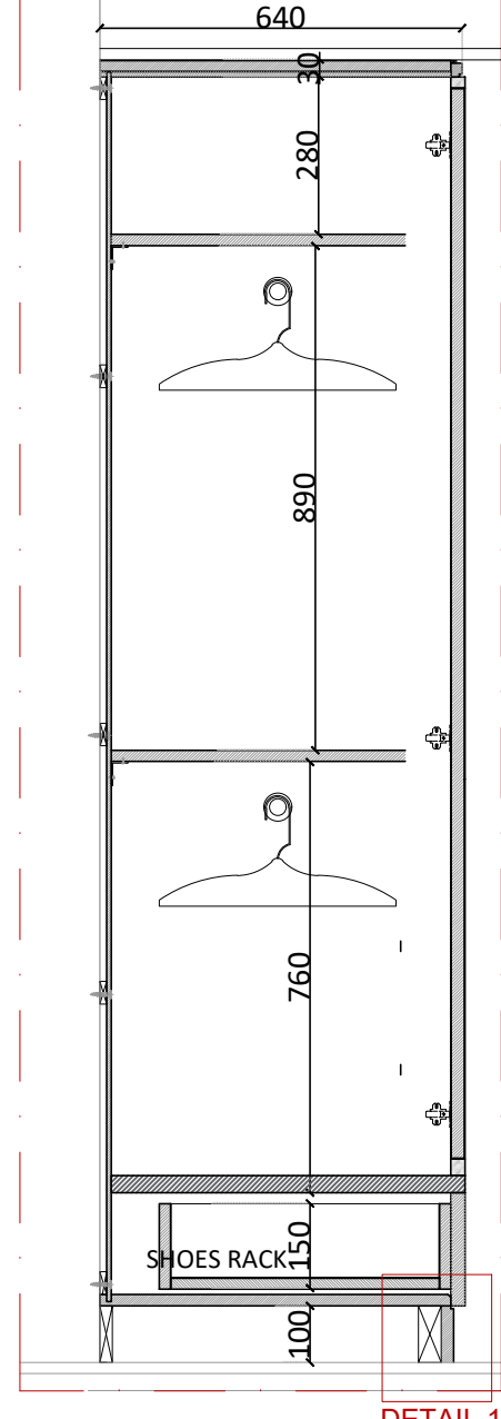
05 SECTION C
