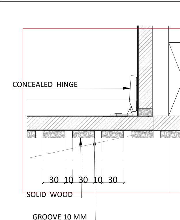
05 Detail 01
